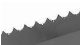
Denture fine pour polystyrène Fine toothting for polystyrene
